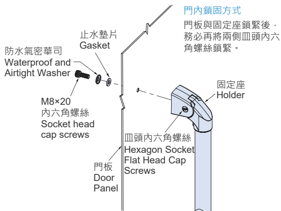
Panels Inner Stationary Type
