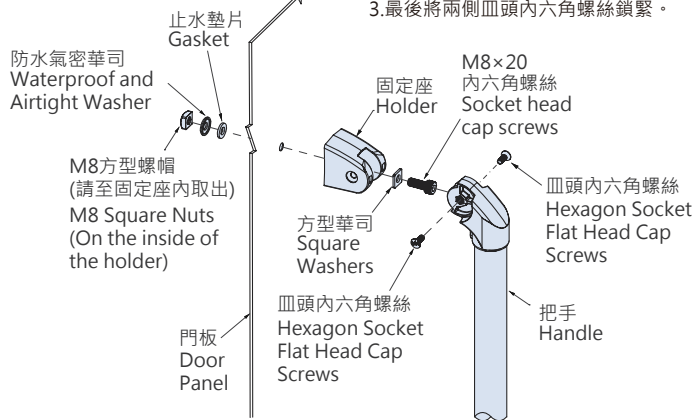
Panels Outside Stationary Type
