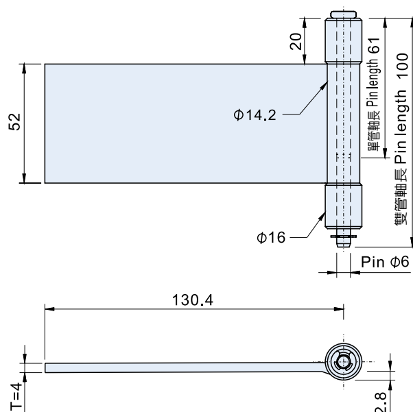
AT-3111 (單管 Single Support)
