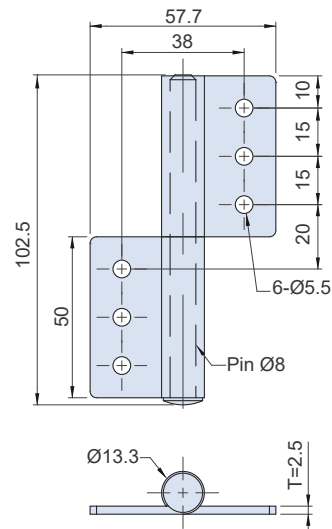
右開有孔型 Right Opening (Screw-on/Rivet-on)
