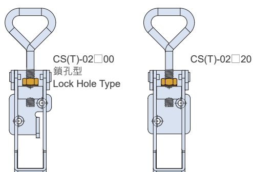
訂製裝配示意圖 Nut & Washer assembly illustration
