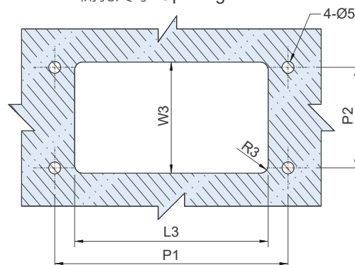
開孔尺寸 Opening size
