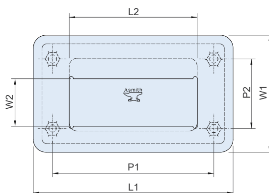
開孔尺寸 Opening size
