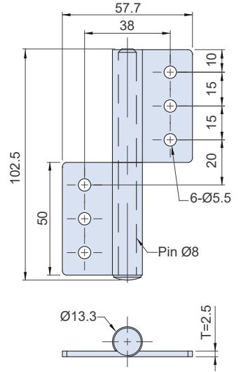
右開有孔型 Right Opening (Screw-on/Rivet-on)
