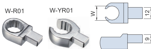
9X12 (開口)梅花式扭力接頭 (Open-)Ring Insert tools
