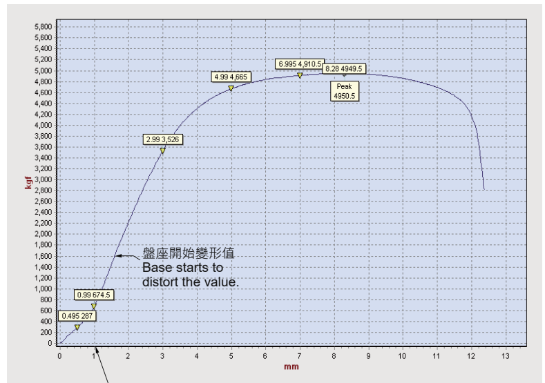
設定荷重 700kgf 下壓值 1 mm。Ø65 圓腳座荷重測試曲線圖 (不含盤墊) Suppose the leveling feet was pressuring under load capacity 700 kgf per 1 mm. The chart show the leveling feet load capacity of bolt and base dimension Ø65 mm.
